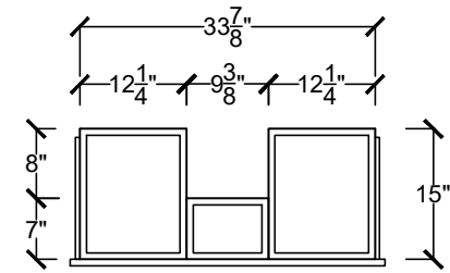
MIDDLE DRAWER BOX DETAIL
