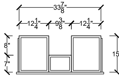
MIDDLE DRAWER BOX DETAIL
