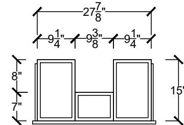
MIDDLE DRAWER BOX DETAIL
